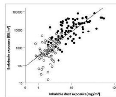
Figure 1. Correlation between 173 personal samples of inhalable dust (mg/m³) and endotoxin (EU/m³) among hand pickers (open circles) and machine room workers (solid circles) in 9 coffee factories.
